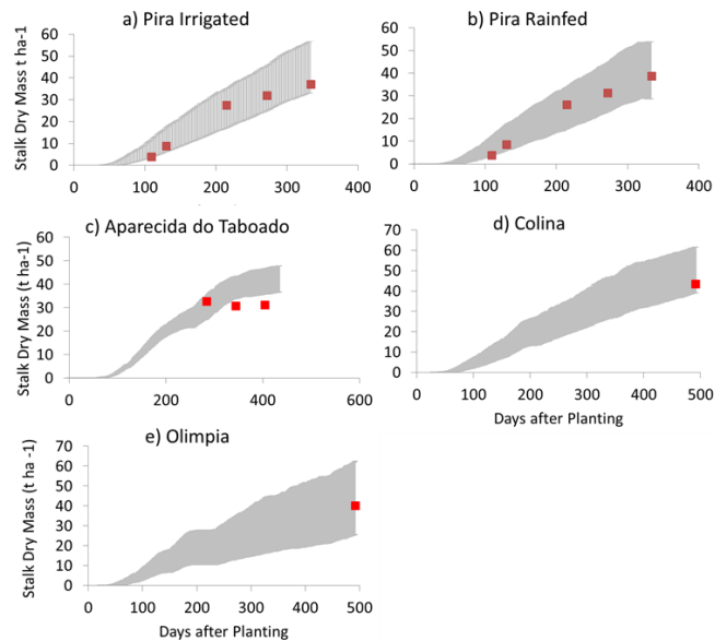
Fig. 2. Time variation of observed and stochastically simulated stalk dry mass for five datasets of cultivar SP83-2847 in Southern Brazil.
